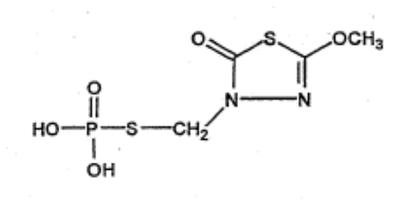
Phosphorthioic acid, 4-(mercaptomethyl)-2-methoxy-1,3,4-thiadiazolin-5-one
