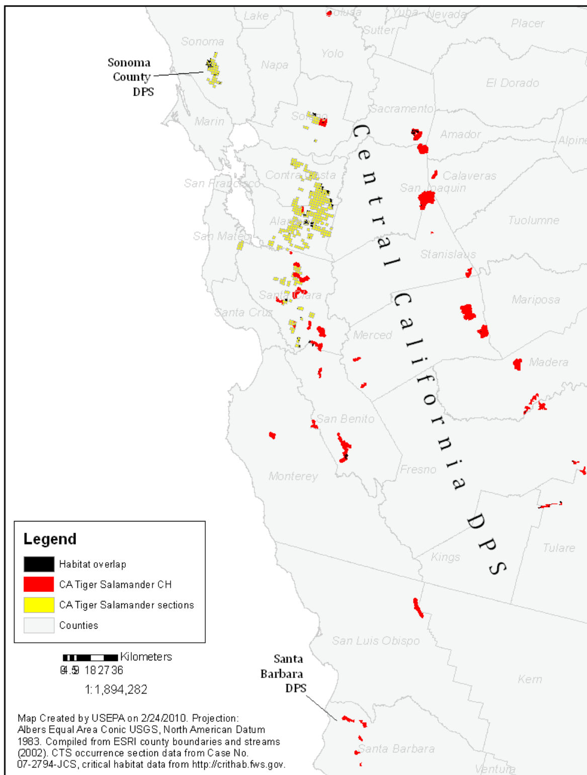
Figure 5 Phosmet potential use (cultivated, orchards/vineyards, pasture) overlap with CTS critical habitat and occurrence sections.
