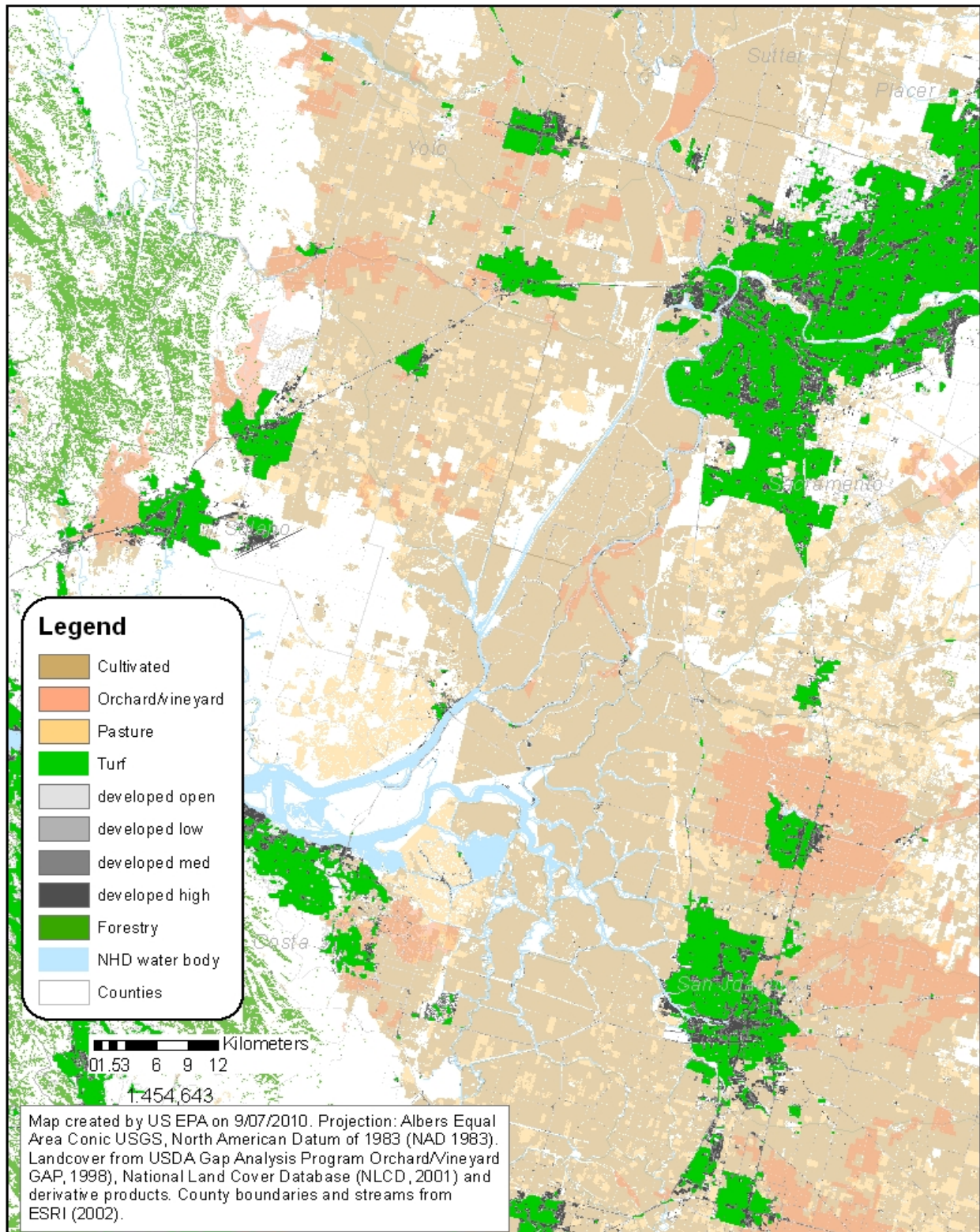
Figure J.2. Potential Use of Permethrin near VELB Habitat and Occurrence Sections based on Land Cover Classes
