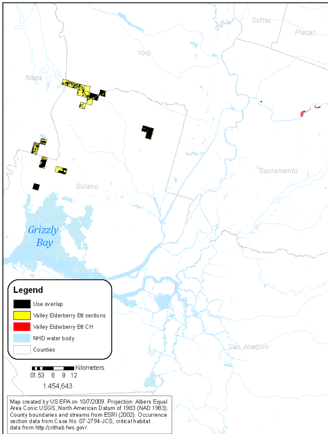
Figure J.3. Overlap of Potential Use of Permethrin near VELB Habitat and Occurrence Sections based on Land Cover Classes
