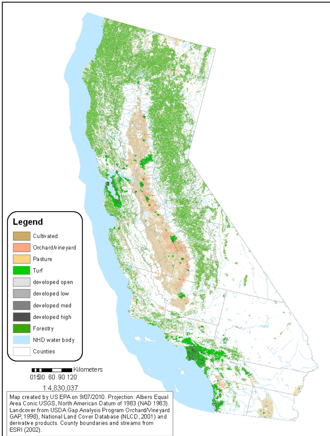
Figure J.1. Potential Statewide Use of Permethrin based on Land Cover Classes
