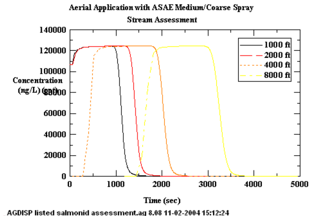
Figure 2. Estimated malathion concentrations over time at various distances downstream from the application.
