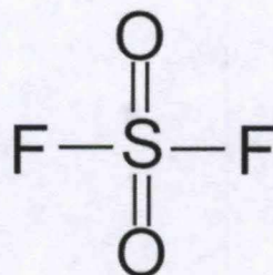
Sulfuryl Fluoride molecular structure
