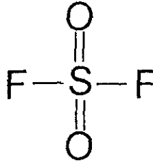
Sulfuryl Fluoride molecular structure
