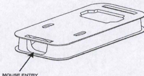
MOUSE BAIT TRAY & LID ASSY. APPROX. DIM.: 2.40" X 5.13" X 1.08" DEPTH
