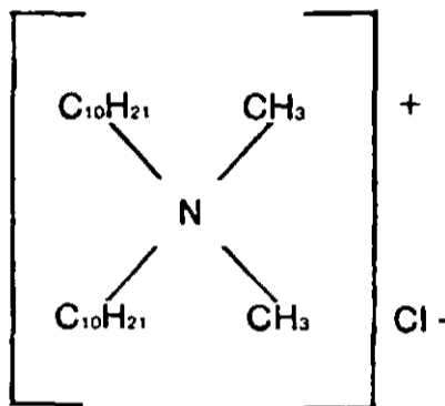
didecyl dimethyl ammonium chloride
