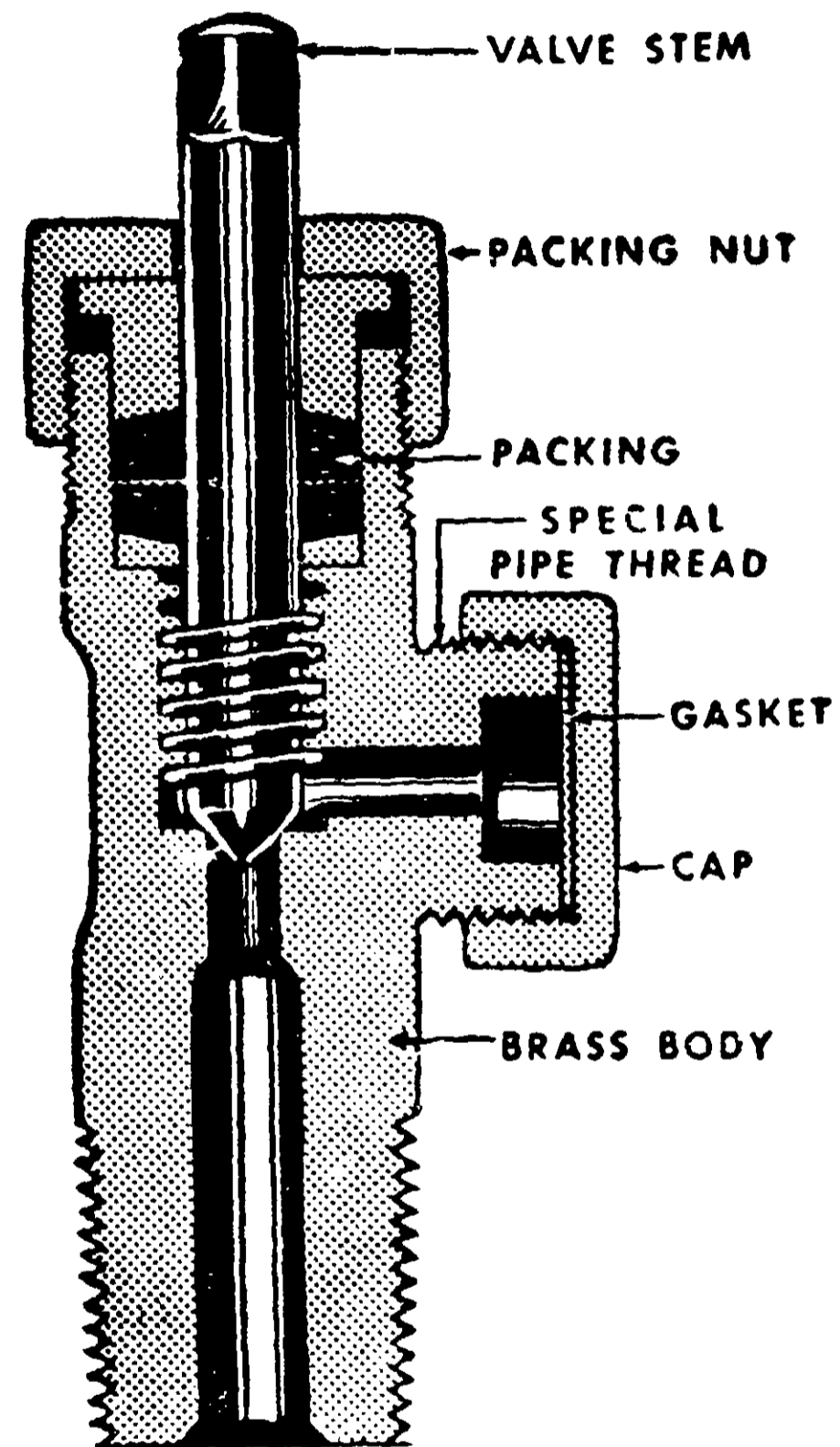
CROSS SECTION OF TON CONTAINER VALVE
