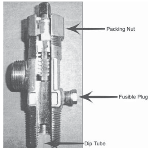
Figure 1. Cylinder Valve
