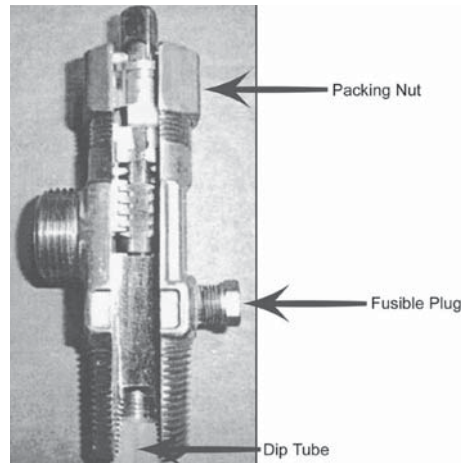
Figure 1. Cylinder Valve
