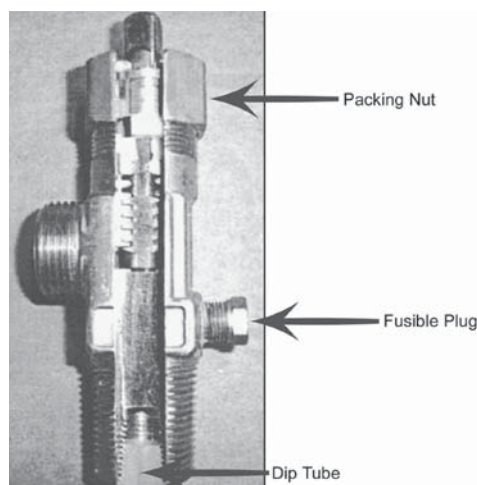
Figure 1. Cylinder Valve
