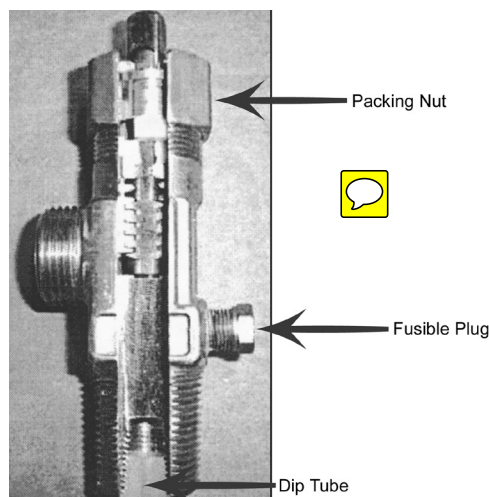
Figure 1. Cylinder Valve
