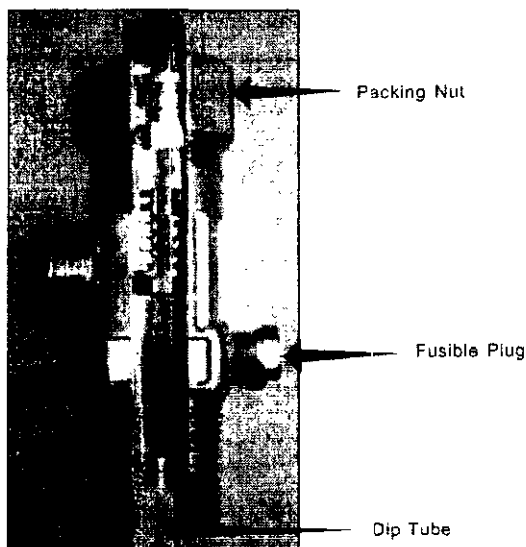
Figure 1. Cylinder Valve
