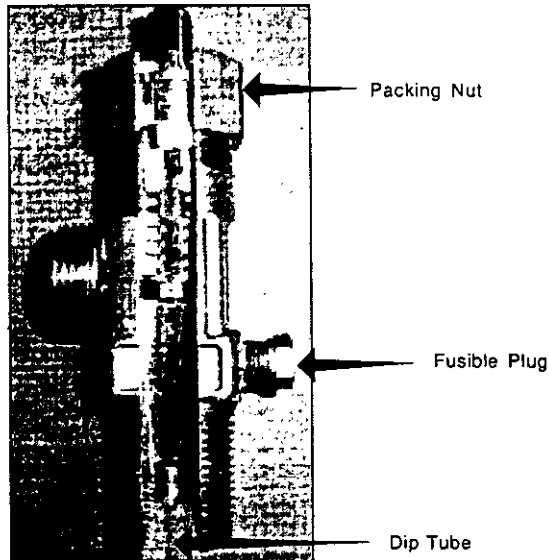
Figure 1. Cylinder Valve
