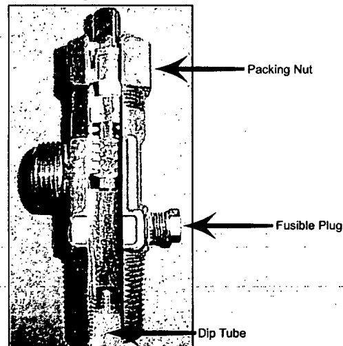
FIGURE 1. Cylinder Valve
