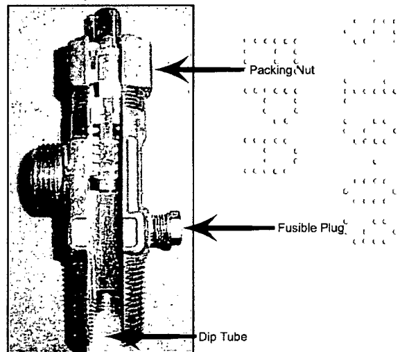
FIGURE 1. Cylinder Valve
