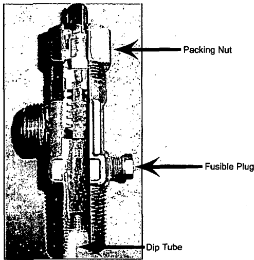
FIGURE 1. Cylinder Valve
