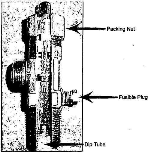
FIGURE 1. Cylinder Valve
