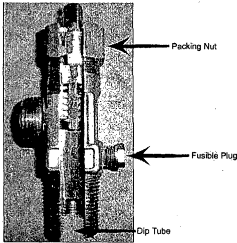
FIGURE 1. Cylinder Valve
