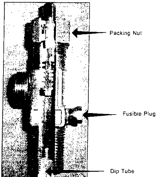
Figure 1. Cylinder Valve
