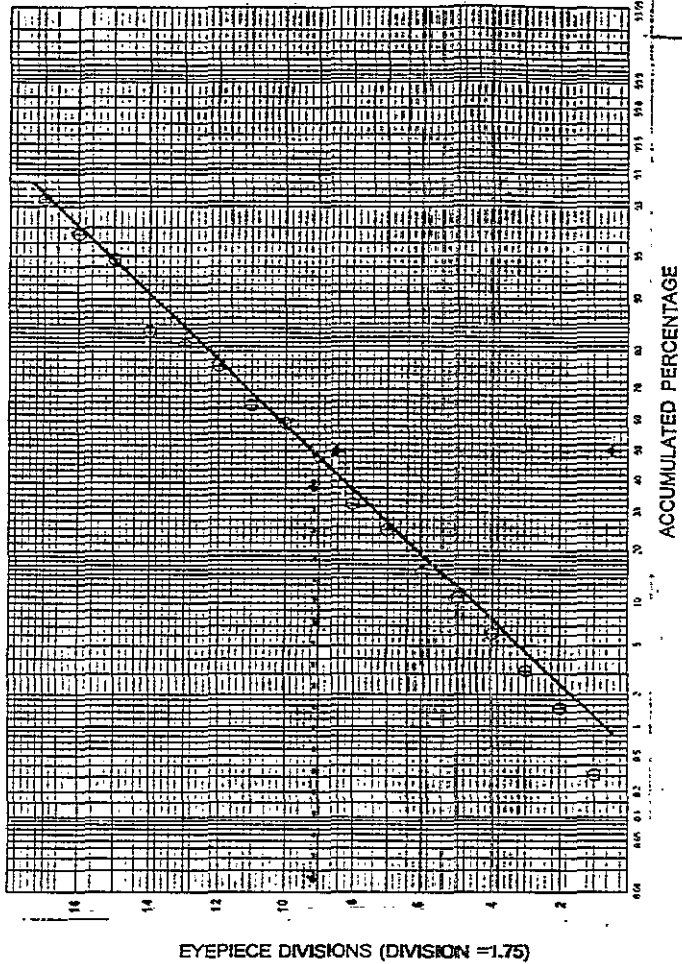
Figure 1 Percentage of the total volume of aerosol samples below each stated droplet size (from Table 1). The Mass Median Diameter is determined from the 50 percent point on the line. The Mass Median Diameter (MMD) = 9.2 divisions times 1.75 =
