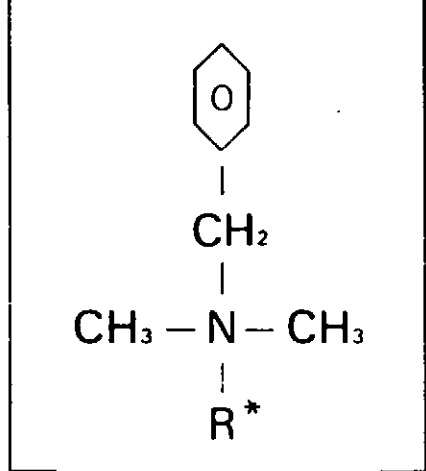
N-Alkyl *(60% C 14 , 30% C 16 , 5% C 12 , 5% C 18 ) dimethyl benzyl ammonium chloride
