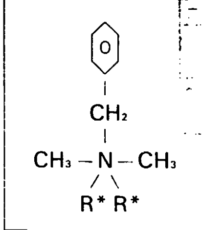
N-Dialkyl *(60% C 14 , 30% C 16 , 5% C 12 , 5% C 18 ) methyl benzyl ammonium chloride
