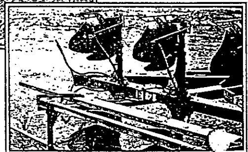
Flip plow with application hoses routed behind the moldboards. A "T" assembly allows the Telone to drop to the opposite set of moldboards when the plow flips over.
