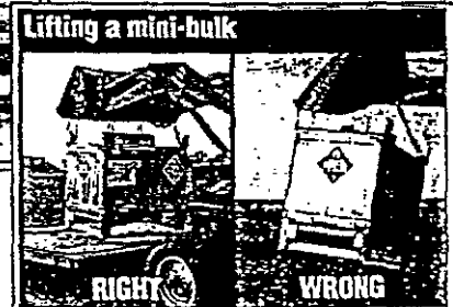
Lifting a mini-bulk Chains must be perpendicular when lifting. DO NOT draw chains into a central point when lifting.
