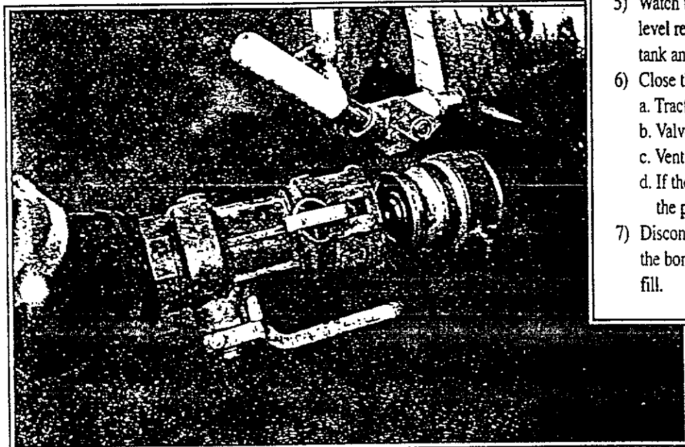
After attaching the electrical bonding cable, connect liquid transfer line with dry-disconnect coupler.
