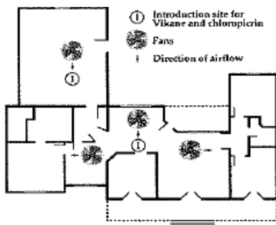
Figure 3. Example of Fans Repositioned for Unidirectional Flow for Aeration of Vikane
