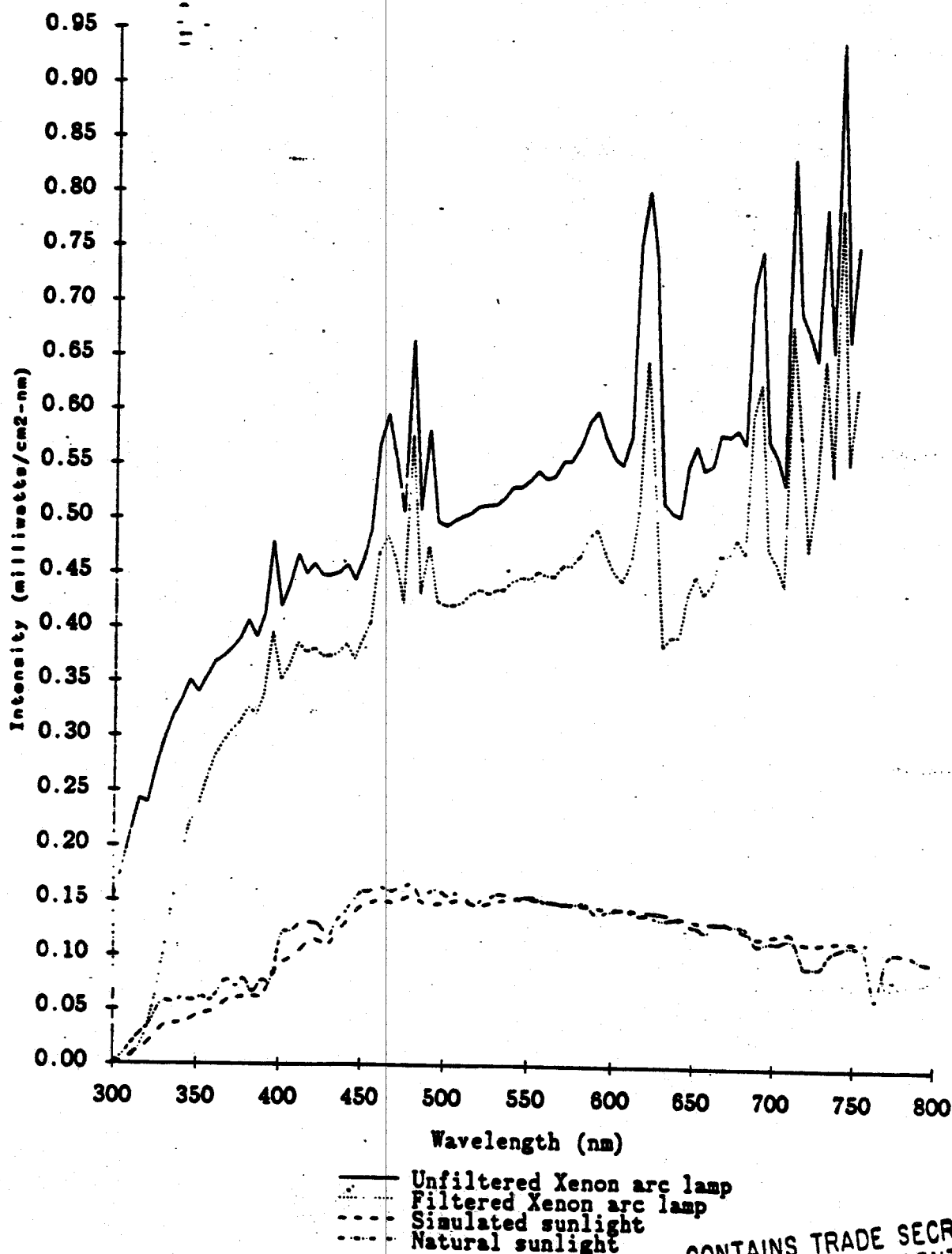
Figure 10. Intensities of Natural Sunlight, Simulated Sunlight, the Unfiltered Lamp, and the Filtered Lamp Used in the MON 13900 Aqueous Photolysis Studies
