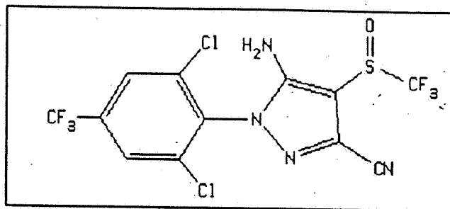
Figure 1 Fipronil
