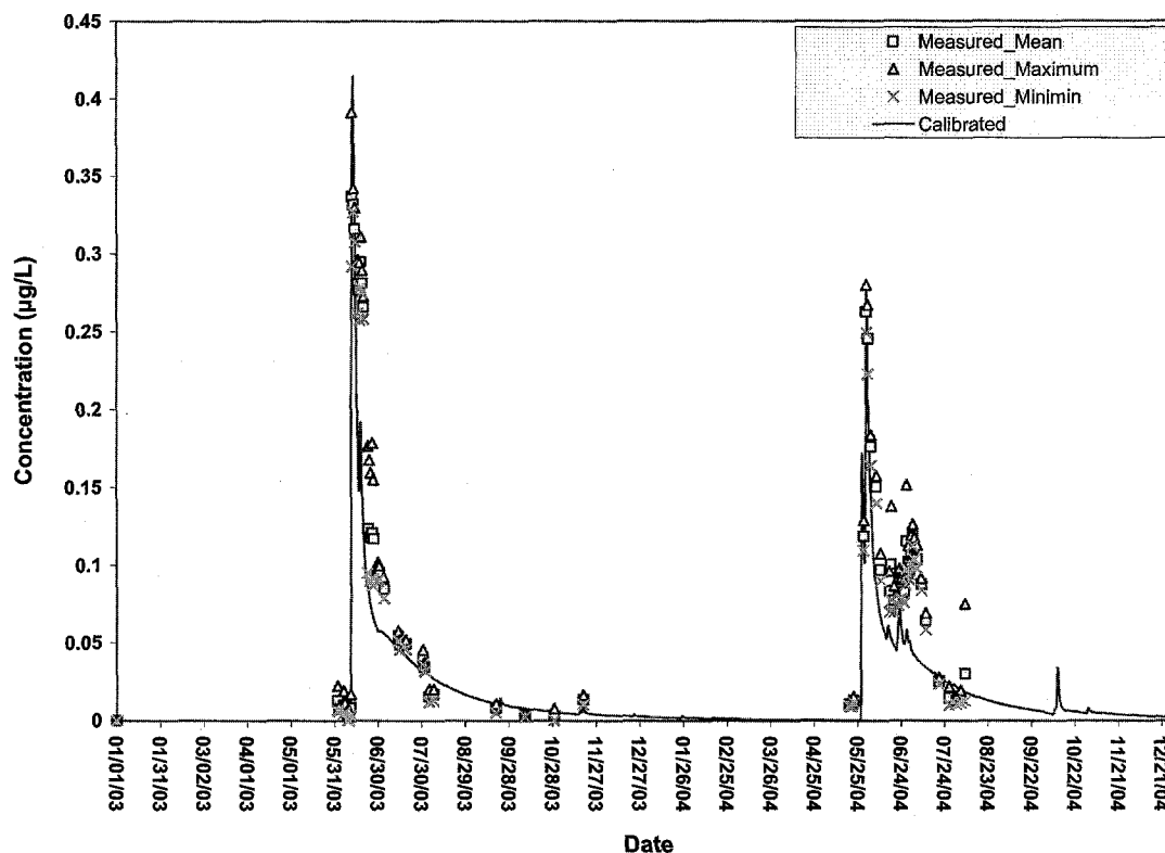
Figure 7 Simulated Total Fiprole Concentrations Compared to the Measured Concentrations in 2003 and 2004
