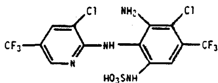
DAPA-sulfamate isomer
