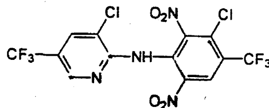
^{14}\text{C}(\text{Py}) -IKF-1216
