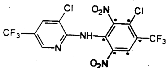
^{14}\text{C}(\text{B}) -IKF-1216
