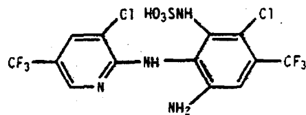
DAPA-sulfamate isomer
