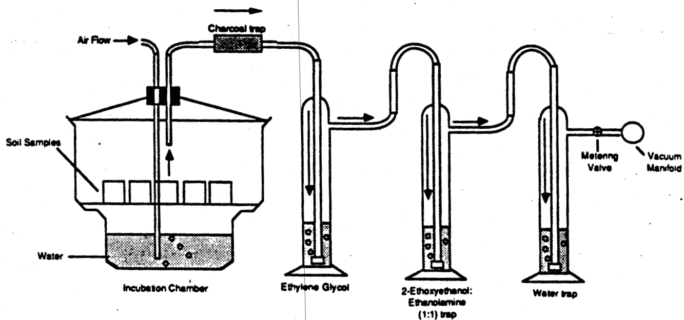
Figure 2. Schematic diagram of the aerobic incubation apparatus used for the test material aging phase.
