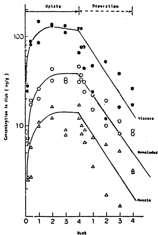
Figure 2. Total radioactivity (ng/g cyhalothrin equivalents) in (a) whole fish and (b) viscera, muscle, and remaining tissues (brains, gill, scales, skin, fins, and skeleton) during the uptake and depuration periods.
