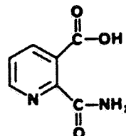
2-Carbamaylnicotinic acid (CL 60,032)
