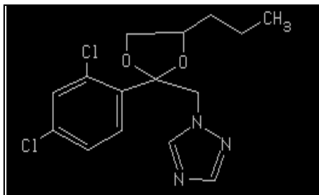
Propiconazole
