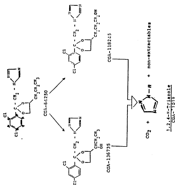
Figure 2: SOIL METABOLISM OF CG:-64250
