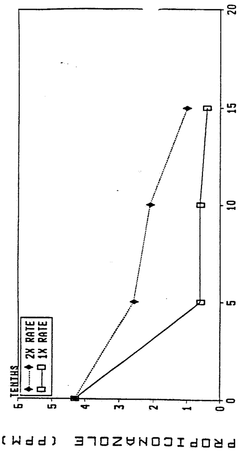
TEXAS FLOOD WATER PROPICONAZOLE
