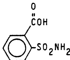
2-(aminosulfonyl)benzoic acid
