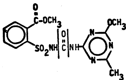
Metsulfuron Methyl
