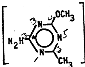
4-methoxy-6-methyl-1,3,5-triazine-2-amine
