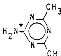
4-amino-6-methyl-1,3,5-triazin-2-ol
