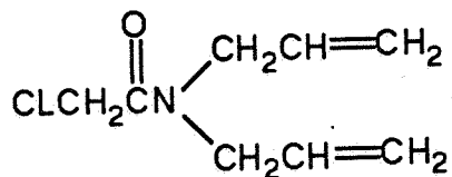
Allidochlor
