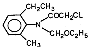
Acetochlor
