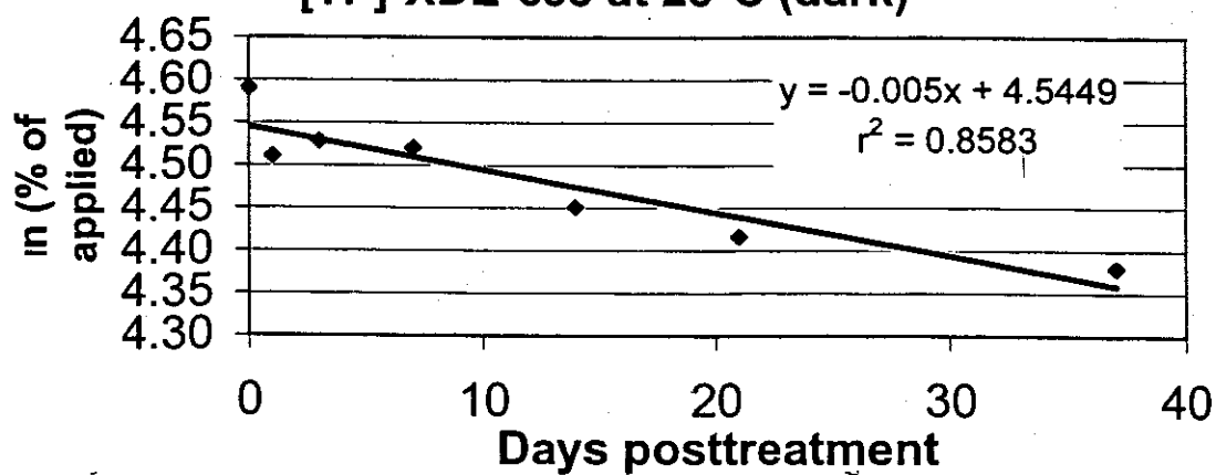
Photodegradation in Arkansas/Amagon soil of [TP]-XDE-638 at 25°C (dark)
