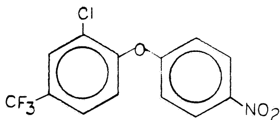
4-[2-Chloro-4-(trifluoromethyl)phenoxy]- 1-nitrobenzene (MC-10074)
