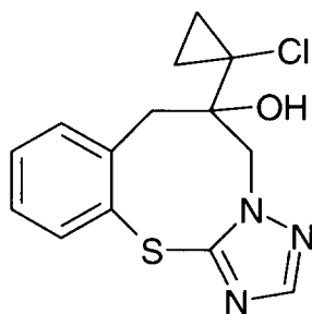
Figure 8. Prothioconazole-thiazocine
