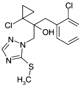
Figure 7. Prothioconazole-S-methyl
