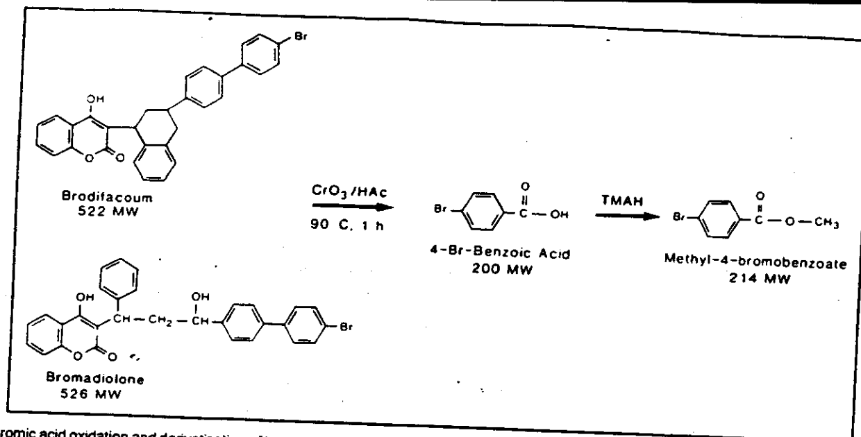
Fig 1—Chromic acid oxidation and derivatization of brodifacoum and bromadiolone. MW = molecular weight; HAc = acetic acid; TMAH = trimethylanilinium hydroxide.
