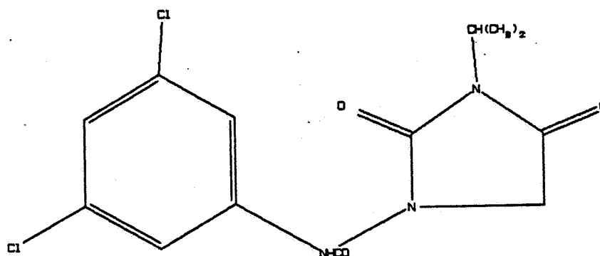
1-(3,5-dichlorophenyl)carbamoyl-3-isopropyl hydantoin RP-30228
