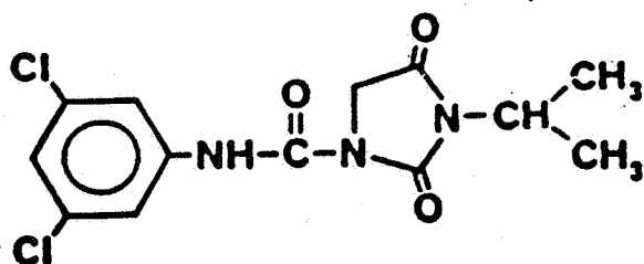
1-(3,5-Dichloroanilino)carbonyl-3-isopropylamino-2,4-dioxoimidazolidine
