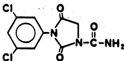
3-(3,5-Dichlorophenyl)-2,4-dioxo-1-imidazolidinecarboxamide
