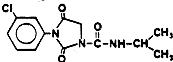
1-Isopropylcarbamoyl-3-(3-chlorophenyl)hydantoin
