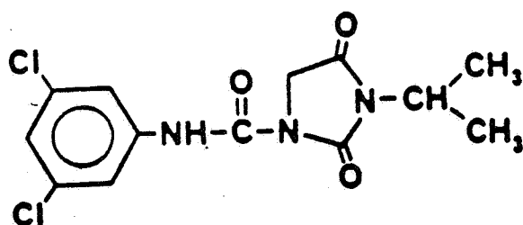
1-(3,5-Dichlorophenyl)carbamoyl-3-isopropylhydantoin (RP-30228)
