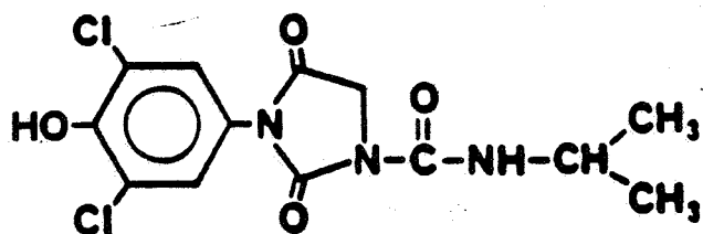
Isopropylcarbamoyl-1-(3,5-Dichloro-4-hydroxyphenyl)-3-hydantoin (RP-37677)
