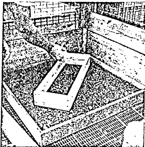
Fig. 1. Application of COUNTER to one of the 76.2 × 76.2 × 7.6-cm (30 × 30 × 3-inch) soil trays. The insecticide was placed in a 17.8-cm (7-inch) band over a hypothetical corn row to simulate normal field applications.
