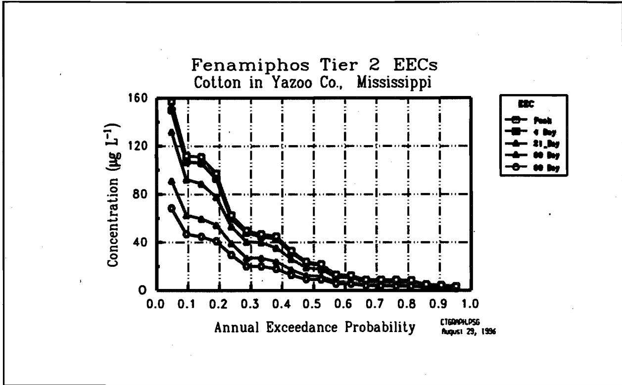
Figure 2. Annual exceedence probability of EEC's for NemaCur 3 on cotton in MS from a single preplant application. Annual maximum concentrations are the greatest concentrations of the given duration which occurred during the year.
