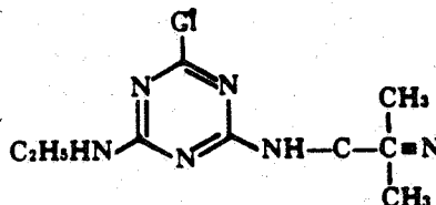
Cyanazine (Bladex)
