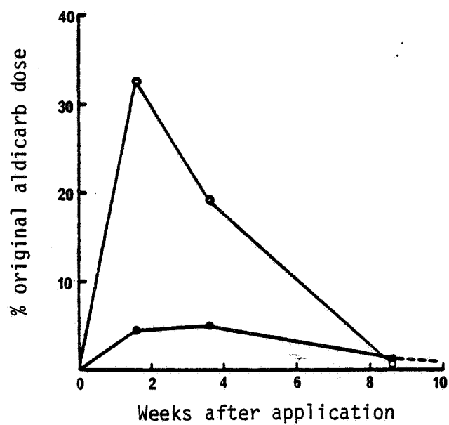
Figure 1. Persistence of the oxidation products of aldicarb in grassland sandy soil o-o, aldicarb sulfoxide; ●-●, aldicarb sulfone.
