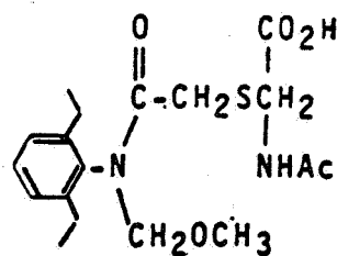
Tertiary Mercapturate (5)
