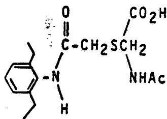
Secondary Mercapturate (4)
