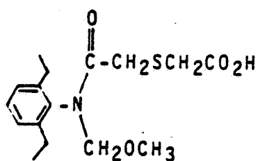
Secondary Mercapturate (4)
